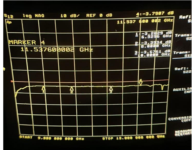
Figure 2 Isolation (Reverse)
