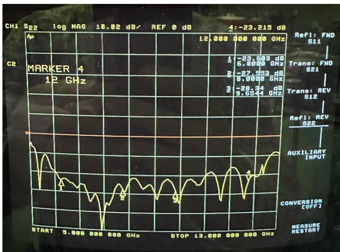
Figure 3 Reflection Coefficient at Port 2
